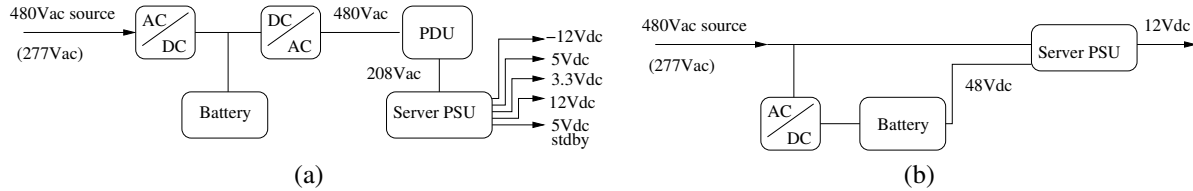
Figure 1. Schematic view of power distribution to the server. Inside the typical datacenter (a), an external three-phase 480Vac source provides power to large UPSs, consisting of rectifiers to convert AC to DC, a battery to store the energy, and an inverter to convert back to AC. Voltage is then transformed to 208Vac through PDUs and distributed to the servers. Each conversion loses some energy, typically around 5%, 5%, and 3%, respectively. Contrast this to our offline design (b), where in normal operation, 277Vac power from the AC source flows through RPPs directly to the PSU with no conversion losses. The battery takes only a fixed amount of charge in normal offline operation, representing only \approx 0.5\% of equivalent system loss. In backup operation, the battery feeds the server PSUs directly with 48Vdc.
