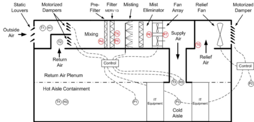
Figure 2. Schematic view of air flow throughout the datacenter. Outside air is pulled in at the top level of the datacenter and cooled by misting, as necessary. Excess moisture is screened out before the cold air is allowed to drop into the cold aisles of the compute floor. The air is pressurized through the server racks to the back, hot aisles (that can be heated above human comfort levels because they require no servicing). The hot air is dumped outside or mixed with incoming air when outside temperatures are too cold. Excess heat can also be used for the office space in the winter. Distributed sensors monitor the environment and adaptively control temperature, moisture, and air pressure in real time.
