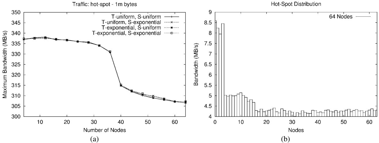
Figure 16. Write hot-spot.
